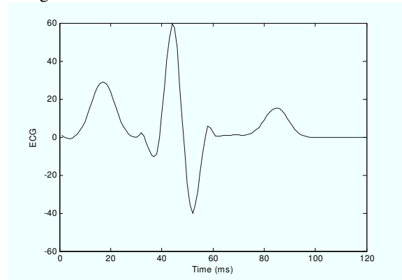
Figure 3 Simulated ECG signal for one beat.
