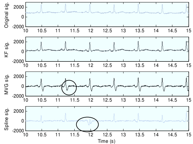
Figure 2 Comparison of the distortion in the signals.
