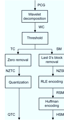
Figure 4. Raw Phonocardiogram Compression (RPC) algorithm.
