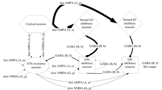
Fig. 2. Block diagram of the population level model of the basal ganglia that is fitted to the PSD of the recorded LFP recordings.
