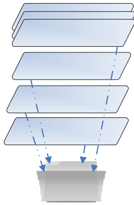
Fig. 1. The accumulation of features per protein/peptide produced by the proteomics analysis steps.
