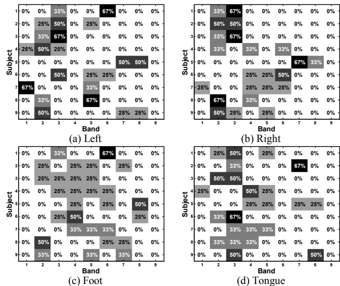
Fig. 4: Histogram of features selected from specific filter bands for each classifier based on the OVR approach using all the training data. The vertical axis in each chart represents Subjects 1 to 9 from top to bottom. The horizontal axis represents the filter bands 1 to 9 from left to right.
