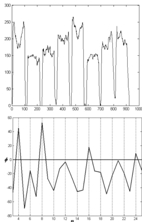
Fig. 2. Cumulative function f (top) and function \phi (bottom), both for test image G1b .
