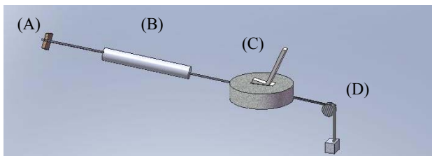
Fig. 1: Schematic diagram of the experimental setup with (A) the string and stopper, (B) string guide, (C) 2 Aquaflex gel pads with cut-out wedge and transducer, and (D) 100 g mass and pulley.
