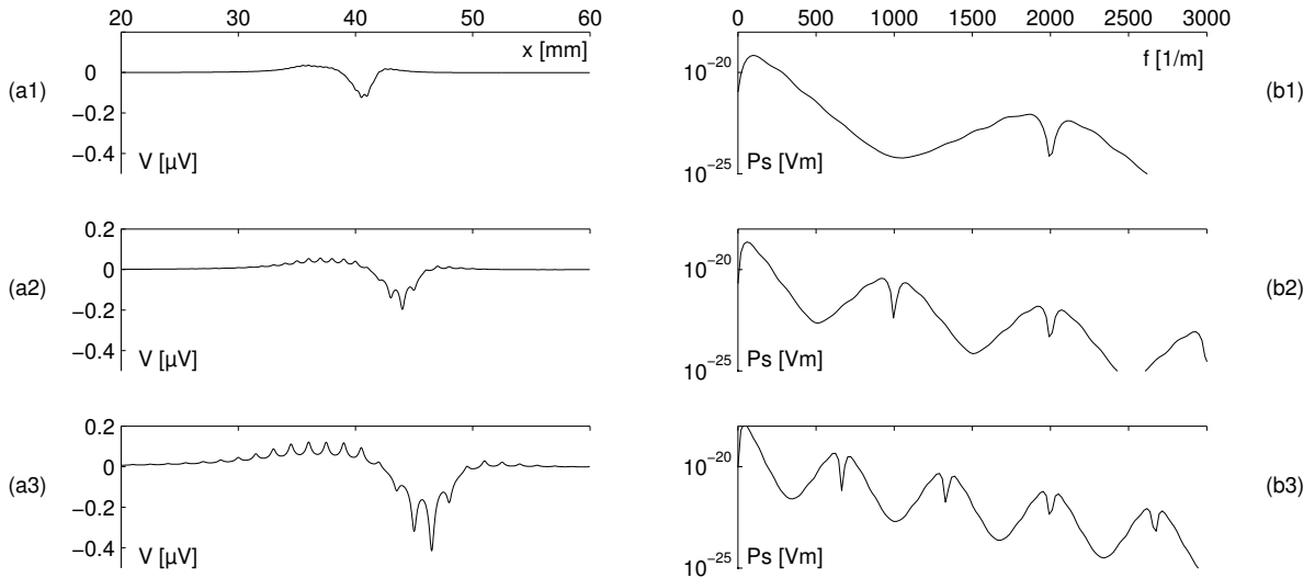
Fig. 2. Extracellular potential plotted along the axon's axis at a distance of 200 \mu\text{m} from the membrane, for different fiber diameters 5.7, 8.7 and 16 \mu\text{m} respectively in (a1), (a2) and (a3). Typical spectrum of the extracellular potential regarding the spatial frequency in the axon's axis direction, for different fiber diameters 5.7, 8.7 and 16 \mu\text{m} represented respectively in (b1), (b2) and (b3).
