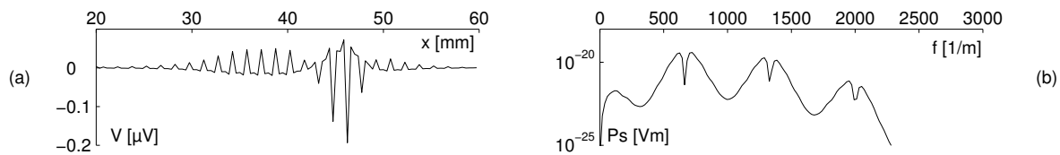
Fig. 5. Laplacian potential plotted along the axon's axis at a distance of 200 \mu\text{m} from the membrane, for fiber diameter 16 \mu\text{m} (a). Typical spectrum of the Laplacian filter output versus the spatial frequency into the axon's axis for this fiber (b).
