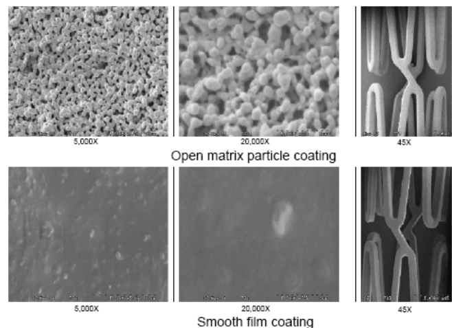
Fig. 1. SEM images of nanocomposite coatings generated by the ElectroNanospray process. Top row is the open matrix coating and the bottom row is the smooth film coating. The column on the right shows the respective coatings applied to coronary stents.
