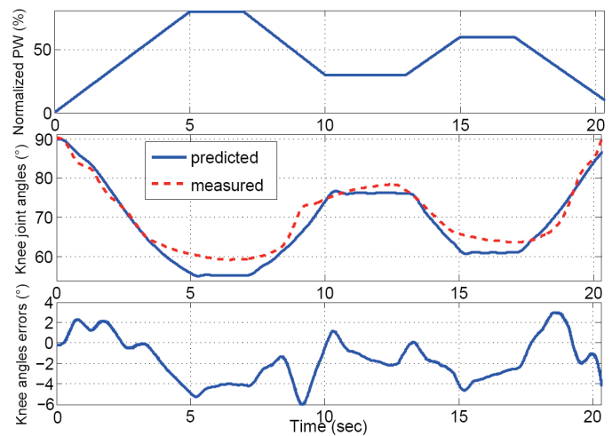
Fig. 5. The cross validation of the complete identified model. (a) Pulse Width ( PW ) of stimulation input. (b) The measured (dashed line) and predicted knee joint angles (solid line). (c) The knee angle errors.
