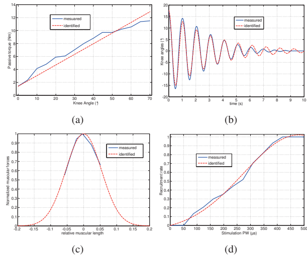
Fig. 3. Identification results: (a) Static passive torque. (b) Passive pendulum test. (c) Force-Length relationship. (d) Recruitment function.
