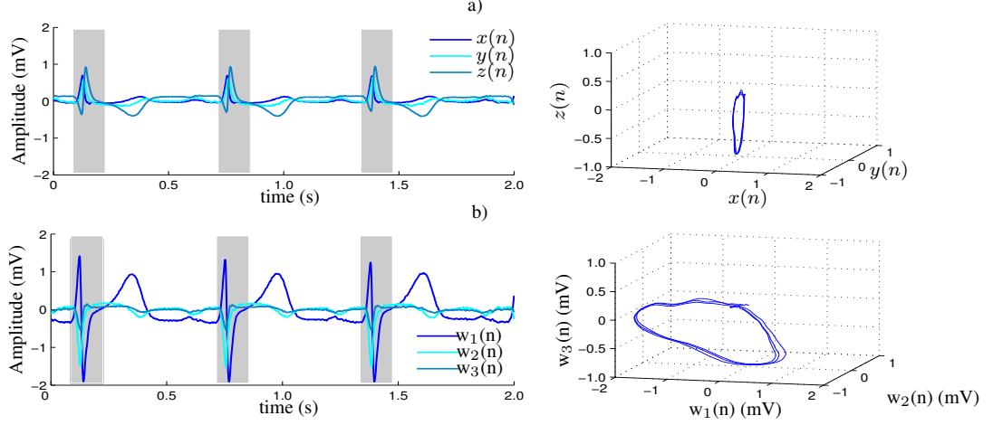
Figure 1. a) Orthogonal X, Y and Z leads derived from Dower Inverse Matrix in a time segment, and their corresponding loops; b) Transformed orthogonal ECG leads obtained from the PCA technique, and their corresponding loops.
