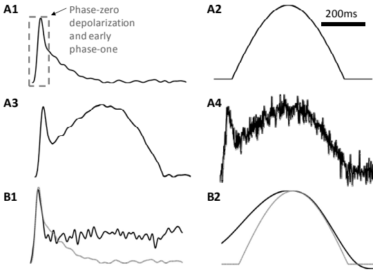
Fig1. Idealized fTmp signals synthesis and analysis. A1 IOAP: ensemble averaged fTmp signal acquired from the epicardial surface of a rat heart after the administration of blebbistatin. A2 Simulated motion artifact: a half-wave rectified sine wave. A3 . Summation of signals in A1 and A2. A4 white noise was added to the signal shown in A3. B1 . Rat IOAP (dotted gray) and reconstructed fTmp signal (rTmp) from detail coefficients at levels 4 to 7 (black). B2 . Simulated motion artifact (dotted gray) and rMA from approximation coefficients at level 7 (black).
