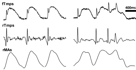
Fig3. Successful reconstructions of OAP phase zero using wavelet analysis. fTmps and rTmps and rMA are shown during pacing (left S1: 700ms) and during an S1-S2-S3 pacing protocol (right). Signals are the average of a 3 pixel radius.
