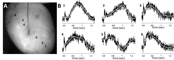
Fig5. Morphology of motion artifact. Motion artifacts were reconstructed using approximation coefficients at level 6 from six different epicardial sites. A. An image of the heart during diastole. The locations of signals shown in B are labeled. B. rMA (gray) is shown on top of original fTmp signals (black) from the six locations marked in A.
