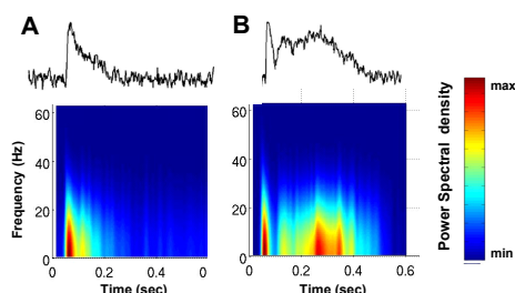
Fig7. Discrete short time Fourier transform analysis of fTmp signals before and after the application of blebbistatin. Spatially averaged fTmp signals (3 pixel radius) are shown above the spectrogram for each signal. A. Spectrogram of an fTmp signal after the administration of blebbistatin (no motion artifact). B. Spectrogram of an fTmp signal before the administration of blebbistatin (with motion artifact). Analysis parameters were window size=32, overlap=31 and NFFT = 1024.
