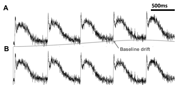
Fig6. Baseline drift reconstruction. A. Spatially averaged fTmp signal using a 3 pixel radius. Baseline drift (gray line) was reconstructed using approximation coefficients at level 10. B. fTmp signal after subtracting the reconstructed baseline drift shown in A.
