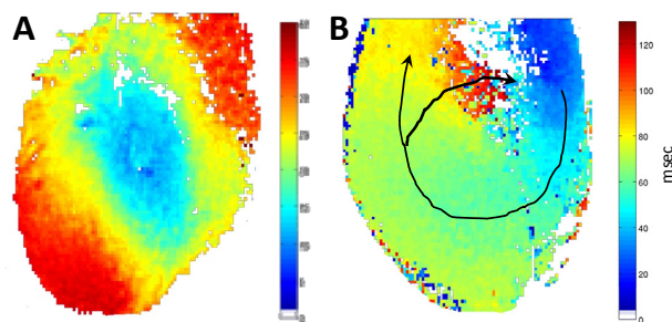
Fig4. Activation time maps for A. paced beat. Wave fronts reveal the elliptical wave originating from the pacing electrode. B. Reentry. Activation times measured from rTmps revealed the reentrant pathway and a slowly conducting zone near the base of the heart.
