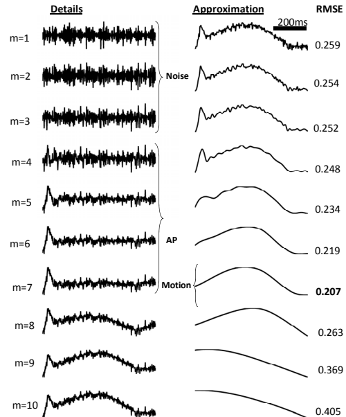
Fig.2 Decomposition of idealized fTmp signal. At each level m signals were reconstructed from detail coefficients d_1 to d_m (left panel) and approximation coefficients a_m (right panel). Lower level detail coefficients represent the noise signal ( m=1 to 3). Approximation coefficients at levels 6 or 7 represent the motion artifact. The RMSE of rMA to the simulated motion artifact ( Fig 1 A1 ) was computed at each level m and are listed on the far left.
