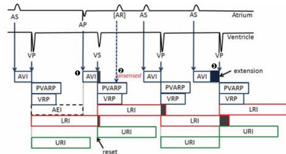
Figure 3. Simulink design of path automata
