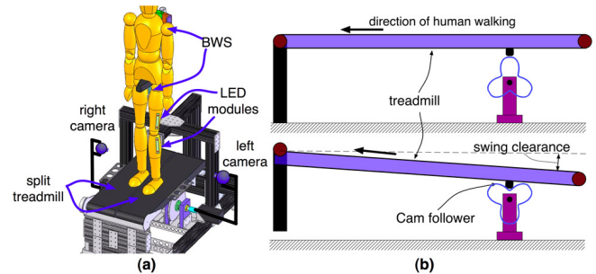
Fig. 1. (a). The MIT-Skywalker platform used for the perturbation experiments. The subject's weight is supported by the body-weight support (BWS) including a saddle-like seat and a chest harness. Two cameras and four LED modules were used for leg motion tracking. (b). Cam-based mechanism of the vertical actuation of the treadmill. As the cam rotates, the follower comes into the low dwell of the cam and a swing clearance of 8.9 cm is created.
