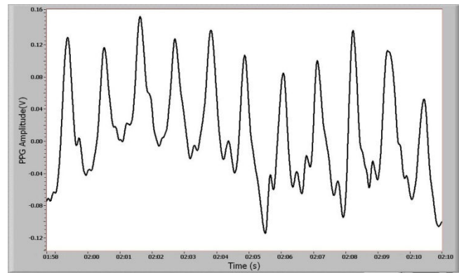
Fig. 3. Pre-operative IR ac PPG from donor site (lower abdomen).
