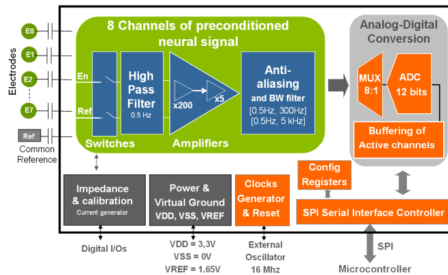
Figure 1: Architecture of the CINESIC8 ASIC
