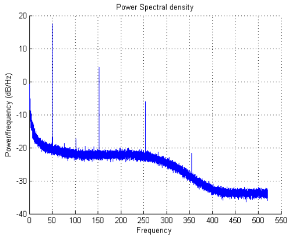
Figure 3: Power spectral density with electrodes set to ground
