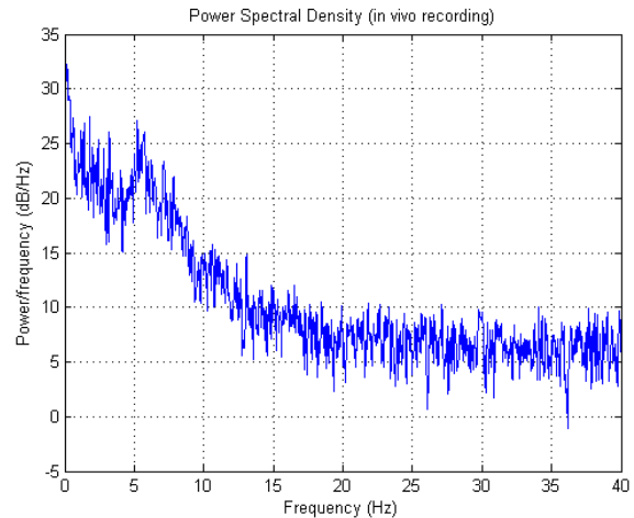
Figure 6: Power spectral density during in vivo experiments
