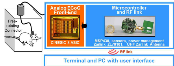
Figure 2: Experimental set-up with ECRINS board and CINESIC8
