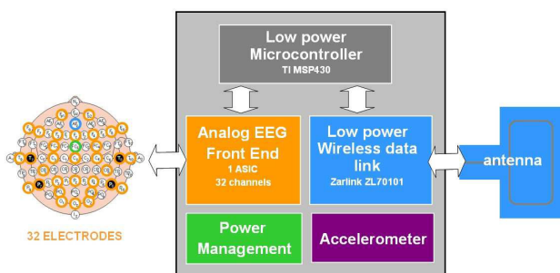
Figure 7: The WIBEEM Architecture
