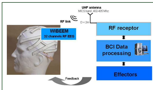
Figure 8: The experimental set-up for WIBEEM
