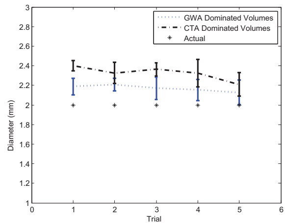
Fig. 4: Tube diameter estimation from 3D ultrasound volumes dominated by two different artifacts: GWA and CTA, with comparison to the known tube diameter.
