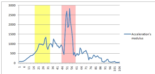
Fig. 4. Acceleration's modulus calculated for backward fall.
