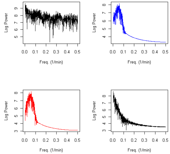
Fig. 3. Power spectra for activity of a resident from the study: the de-meaned original activity signal (top left), the signal filtered with Gabor filters with orthogonal components (top right and bottom left) and the de-meaned combined Gabor energy filter (bottom right.)
