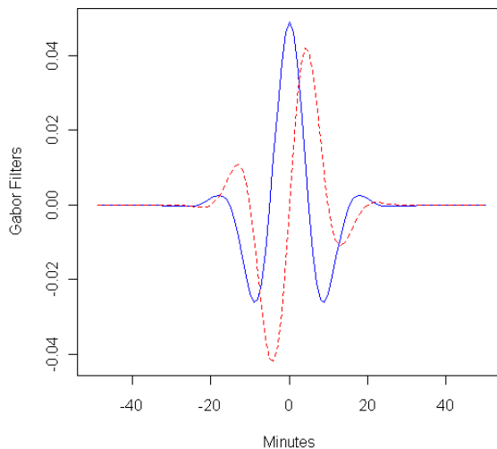
Fig. 2. Gabor filters designed for turn-recognition. The two curves correspond to orthogonal cosine (solid curve) and sine (dashed curve) components.
