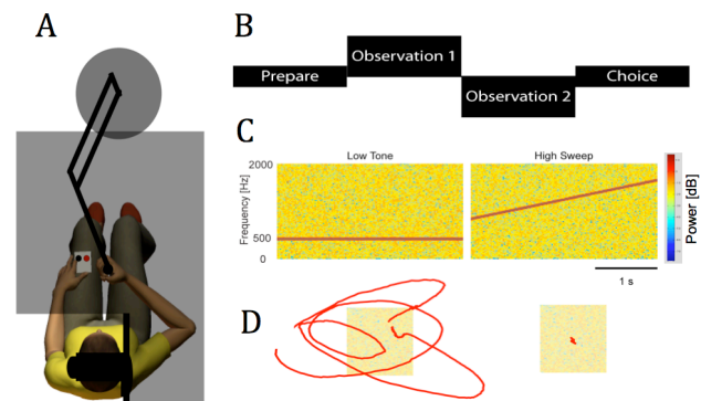
Fig. 1 A: Experimental setup. B: Sequence of events in both the auditory discrimination task and the motion detection task. C: Auditory stimuli. D: Displacement stimuli (left: 1 cm motion; right: no motion).
