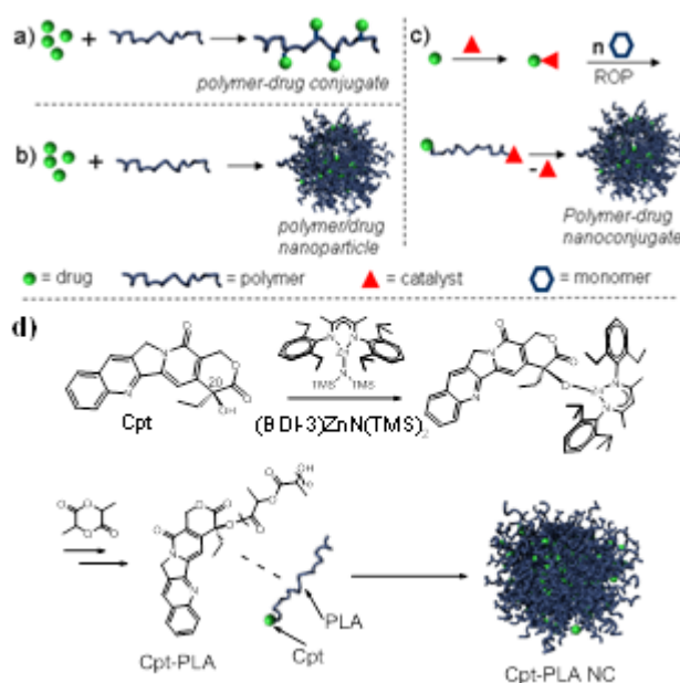
Scheme 1. Illustration of (a) polymer-drug conjugate, (b) polymer/drug nanoparticle, and (c) polymer-drug nanoconjugate via drug-initiated ROP followed by nanoprecipitation. (d) Preparation of Cpt-PLA conjugate through Cpt/(BDI-3)ZnN(TMS) 2 initiated LA ROP.
