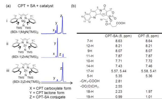
Fig. 1. (a) HPLC analysis of the reaction of SA and Cpt in the presence of (i) (BDI-1)MgN(TMS) 2 , (ii) (BDI-1)ZnN(TMS) 2 , (iii) (BDI-3)ZnN(TMS) 2 ; (b) The chemical shift values of Cpt and Cpt-SA derived from the corresponding 1 H-NMR spectra
