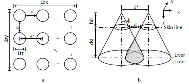
Fig.3.a) Proposed configuration of the multi-transducer system. b) Representation of field of view for two adjacent transducers and the overlapping region.
