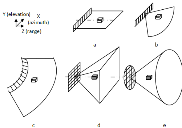
Fig.2. Different types of transducers and the region that can monitor: a) linear arrays, b) 1D phased arrays, c) curved arrays d) 2D phased arrays (square) and e) 2D phased circular arrays
