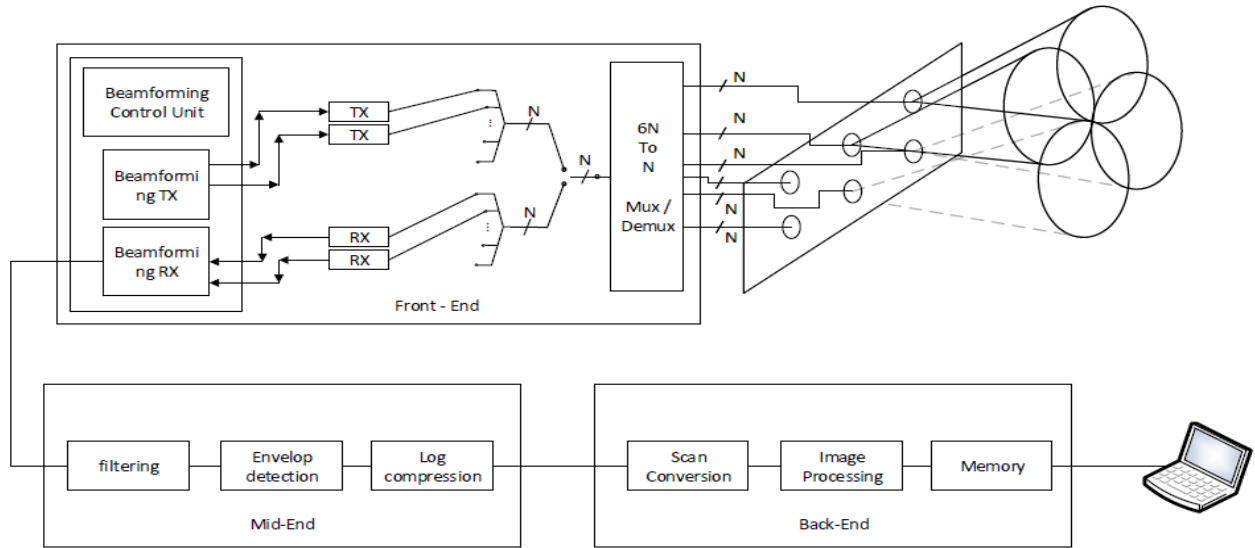
Fig. 4. General architecture of proposed system. Front-end illustrates the integration of the transducers to the board as well as the PSA technique for number of channels reduction adopted from [21]
