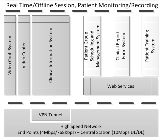
Figure 2: Services Architecture
