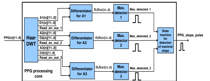
Fig. 9. Internal structure of PPG slope detection core.
