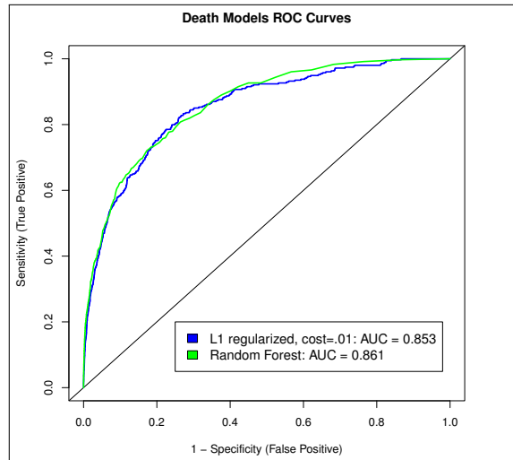
Fig. 2: Death ROC Curves
