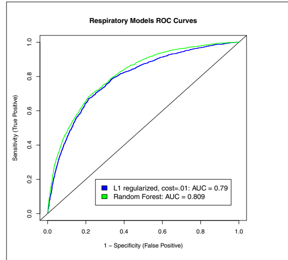
Fig. 9: Respiratory ROC curves
