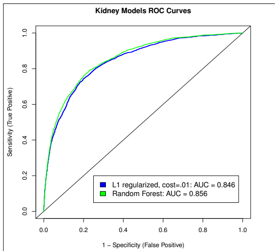
Fig. 5: Kidney Injury ROC curves
