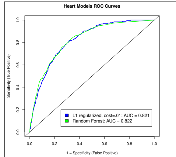
Fig. 6: Heart Injury ROC curves
