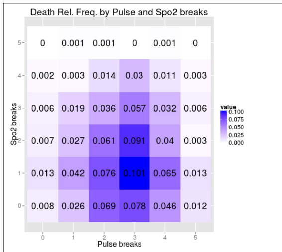
Fig. 4: Death relative frequency by pulse and SpO 2 % breaks
