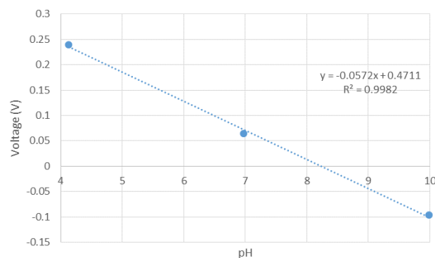
Figure 3. Response of a printed pH electrode each point was recorded with a 10 \mu L sample size of pH buffer solution.
