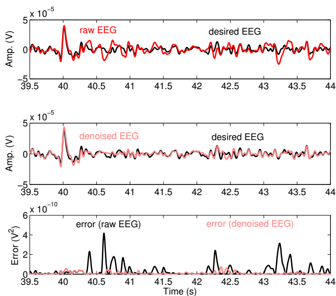
Fig. 5. Motion artefact removal. Top panel: clean/desired and corrupted EEG signals. Middle panel: desired and denoised EEG signals. Lower panel: the squared error prior to and after denoising.
