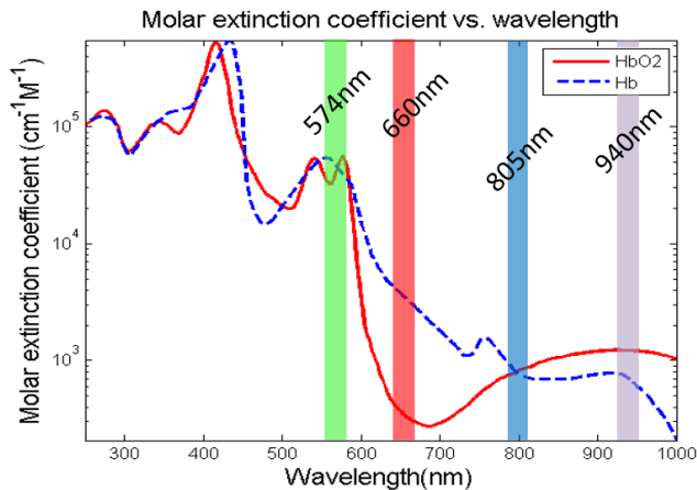
Figure 3. Extinction coefficients for deoxygenated and oxygenated hemoglobin
