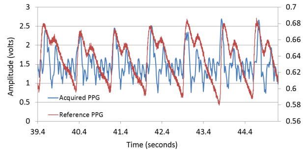
Figure 7. Sample PPG wirelessly acquired from the radial artery via Bluetooth using SoliBand. The periodic noise seen on the signal is noise introduced by the energy harvesting circuit.
