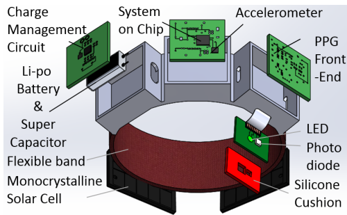
Figure 6. Exploded view of all the components of the device.
