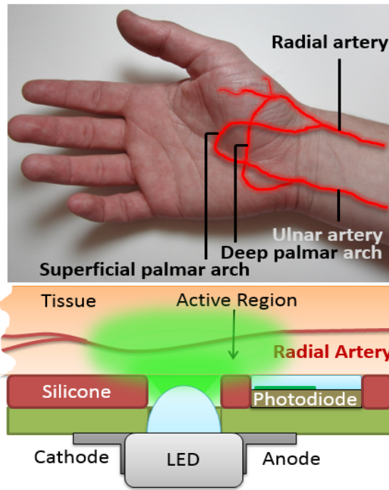
Figure 2. A low profile probe is obtained by use of reverse mount LED. Probe sits atop the radial artery just before the branches to the palmar arches.
