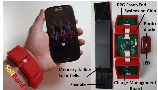
Figure 1. (Left) PPG data being displayed on a smart phone. (Right) The opened device with probe board extended far right for display.
