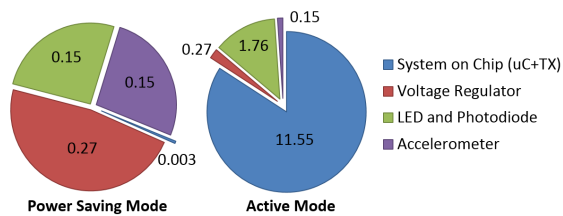
Figure 9. Power consumption in mW for both proposed power schemes
