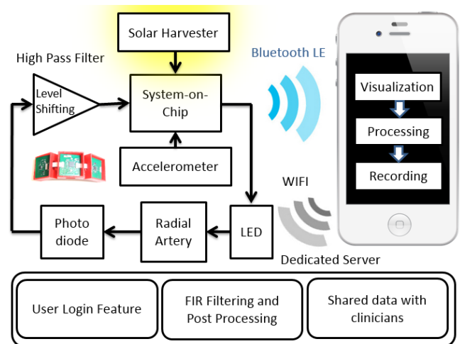
Figure 5. System diagram showing the flow of data from the wristband to the server.
