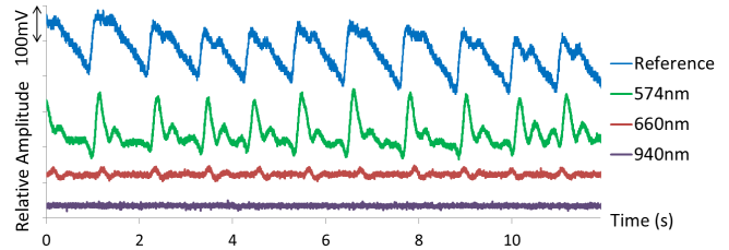
Figure 4. PPG measurement from radial artery with 0.4 mA sent to LEDs with wavelengths in green, red and infrared regions. The reference waveform was obtained using a standard transmittance finger probe (805nm).
