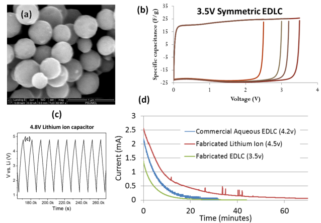
Figure 10. (a) SEM micrograph of high surface area carbon spheres, (b) Cyclic voltammogram of 3.5v EDLC fabricated using the carbon sphere electrodes and (c) Constant current charge/discharge measurements of lithium ion capacitor made using the carbon sphere electrode capable of being cycled to 4.8v at 0.1 A/g (d) Capacitor current discharge profiles for the fabricated single cell capacitors and a commercial five cell capacitor. Each capacitor was charged to capacity under galvanic conditions and connected in parallel to an LED with a 1kohm current limiting resistor.
