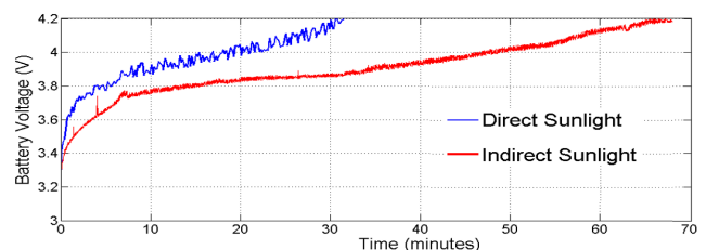
Figure 8. Battery charging profile for indirect and direct sunlight.
