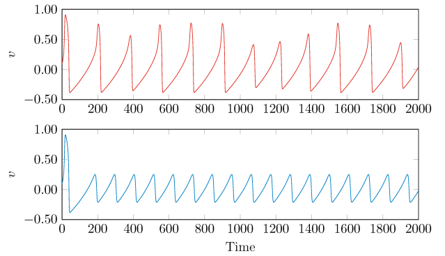
Fig. 1. Different v due to numerical integration tolerance error, fourth-order Runge-Kutta method. Upper figure with RelTol: 1e-3 and AbsTol: 1e-6; lower figure with RelTol: 1e-7 and AbsTol: 1e-10. Parameters : \alpha = 0.008 (upper figure), \alpha = -0.008 (lower figure), \gamma = 0.008 , \varepsilon = 0.01 ; initial conditions : v_{ini} = 0.1 , w_{ini} = 0 ; adaptive time step.
