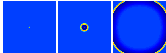
Fig. 5. \alpha = -0.1 (upper) : center stimulation, I_{stim}(100, 100) = 1
