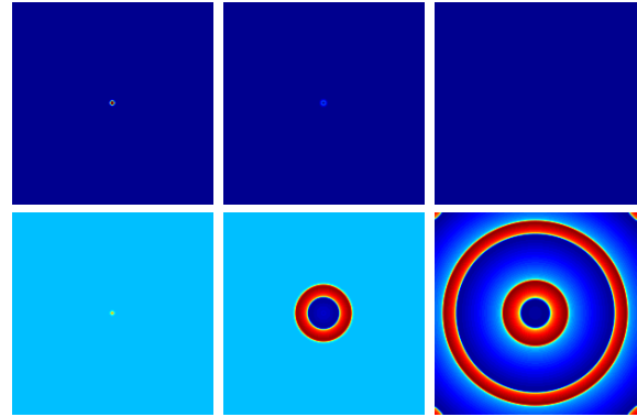
Fig. 4. \alpha = 0.1 (upper) and \alpha = -0.1 (lower), center initiation : v_{ini}(100, 100) = 1 , zeros for other cells; w_{ini}(1 : 200, 1 : 200) = 0 .
