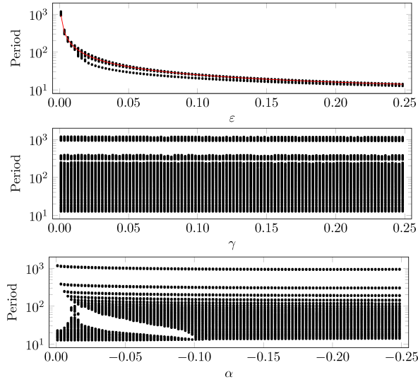
Fig. 6. Parameters' influence on period of AP in FHN. Red curve in first sub-figure is the fitted curve : \text{Period} = 3.065 \times \varepsilon_{\alpha,\gamma}^{-0.8275} + 4.397 . (discontinuity in third sub-figure means no valid AP generated.)
