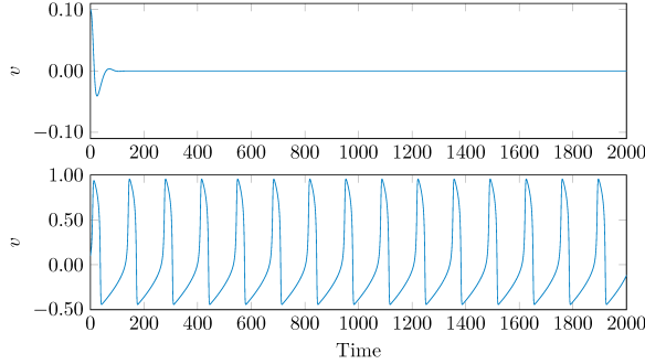
Fig. 2. Comparison of \alpha = 0.1 (upper) and \alpha = -0.1 (lower) in FHN model (Eq. (5)). Parameters : \gamma = 0.008 , \varepsilon = 0.01 ; initial conditions : v_{ini} = 0.1 , w_{ini} = 0 ; adaptive time step.
