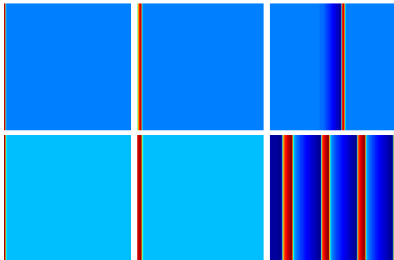
Fig. 3. \alpha = 0.1 (upper) and \alpha = -0.1 (lower), border initiation : v_{ini}(1, 1 : 200) = 1 , zeros for other cells; w_{ini}(1 : 200, 1 : 200) = 0 .
