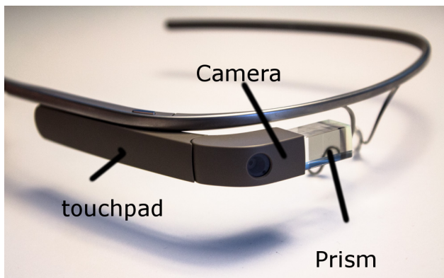
Fig. 1: The Google Glass and their main components.
