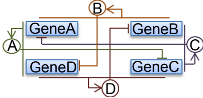
Fig. 4. Two coupled toggle switch network
