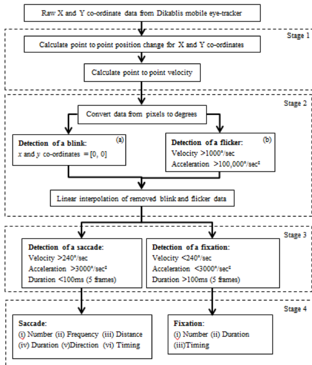
Figure 3. Algorithm flow chat
