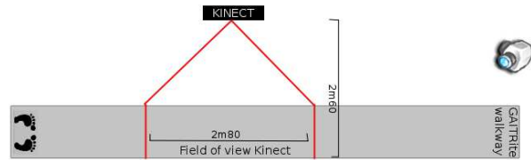
Fig. 3. Measurement set-up
