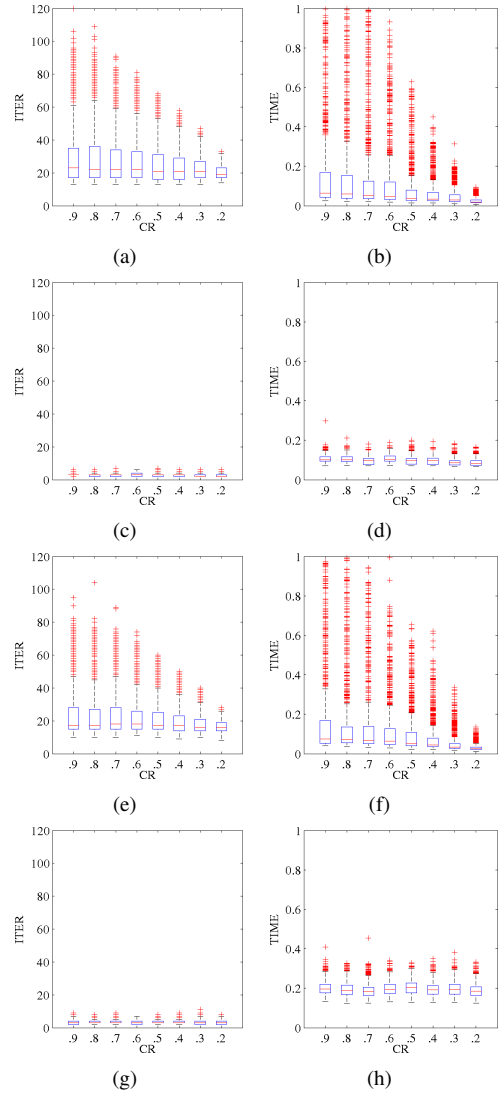
Fig. 1: Number of iterations (left) and processing times (right) until convergence of ((a),(b)) SOMMP, ((c),(d)) S-GAP, ((e),(f)) OMMP and ((g),(h)) GAP as function of CR.
